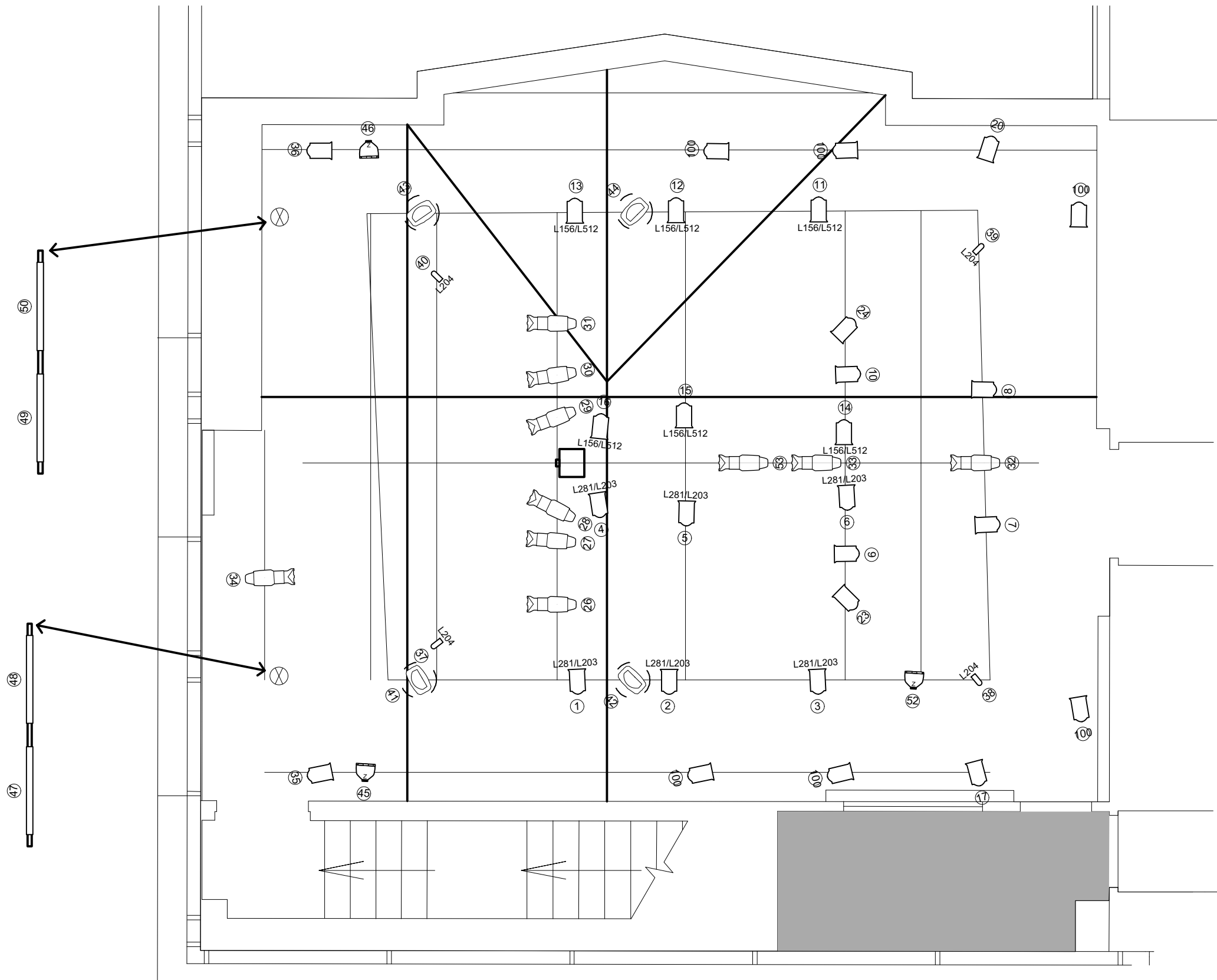
1 Lx Master Plan Scale: 1:50
